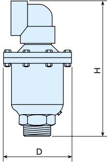
Metallic Body
