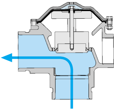
Normal filter flow
