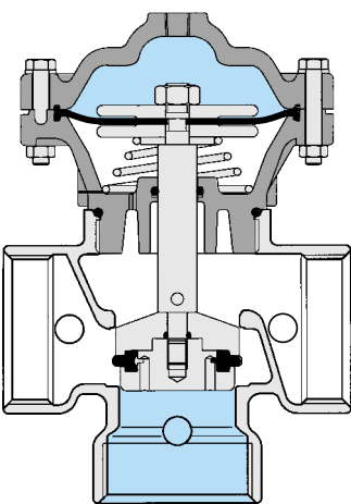
Intermediate stage (change of condition). No water exchange between openings
