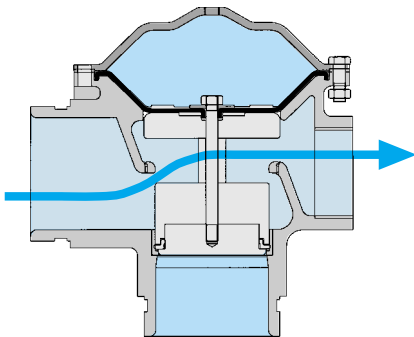
Backwash flow
