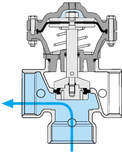
Normal filter flow
