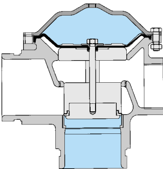
Intermediate stage (change of condition). No water exchange between openings
