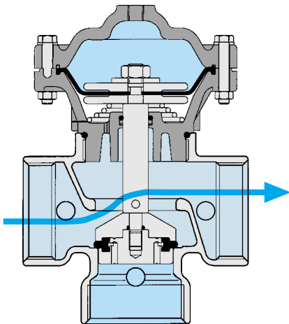
Backwash flow
